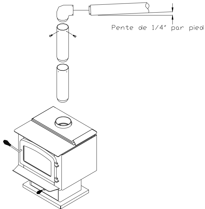
FIGURE 2.3 (B) Pente minimum
