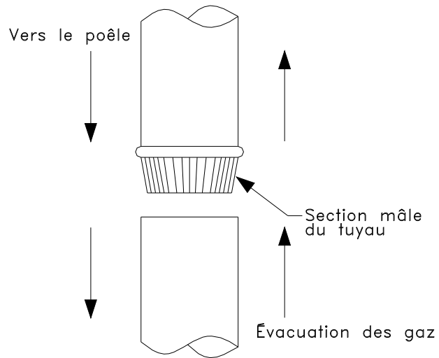
FIGURE 2.3 (A) Raccordement des sections
